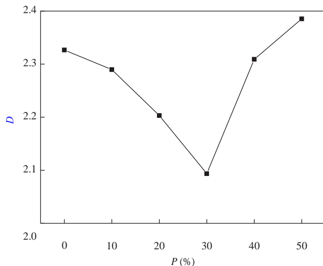
Figure 13: Relationship between the fractal dimension and fly ash contents.
