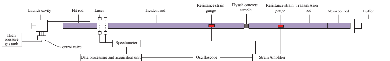
Figure 4: The split Hopkinson pressure bar test system.
