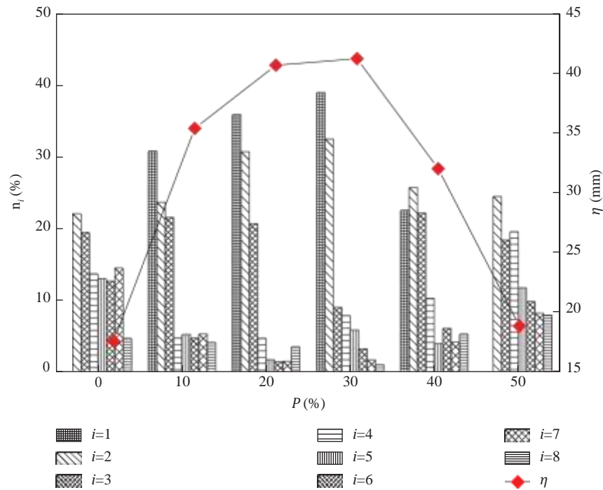
Figure 11: Fragment distribution of concrete with diferent fly ash contents.
