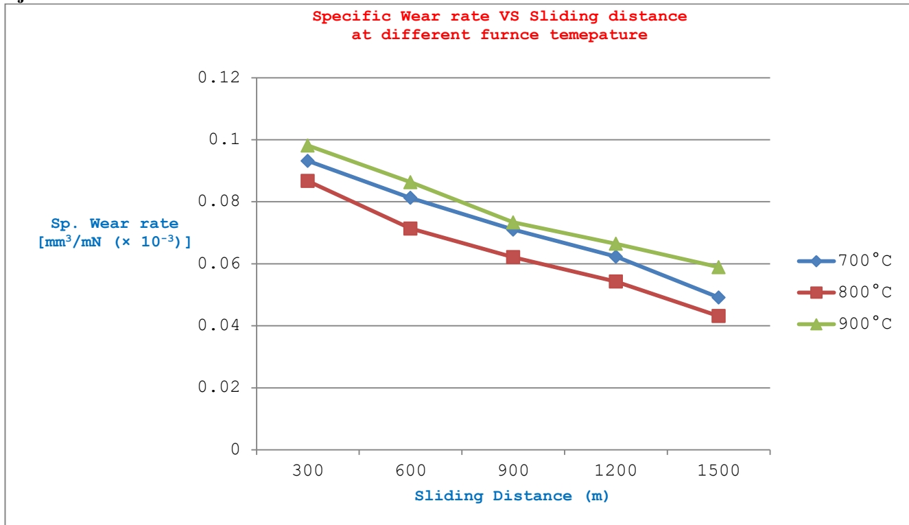
Figure-iii: Variation Sp. Wear Rate at different sliding distance and at different furnace temperature
