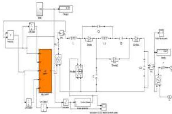
Fig 2 MPPT model
