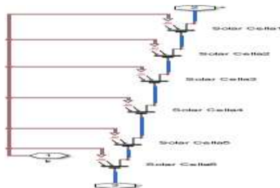
Fig.3 Solar cell
