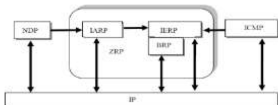
Figure - Complete block diagram of ZRP
